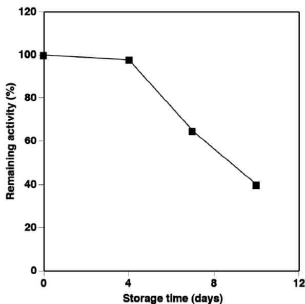
Fig. 4: Evaluation of the stability of homocholine dehydrogenase during storage at 4°C.
