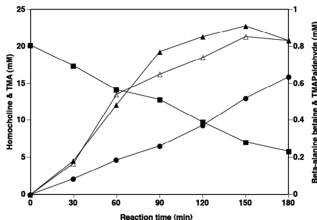
Fig. 5: Degradation of homocholine by resting cells of Pseudomonas sp. strain A9. Time course degradation of homocholine (■) and the generation of the metabolites, TMAPaldehyde (△) beta-alanine betaine (▲) and TMA (●) by intact cells of Pseudomonas sp. strains A9.
