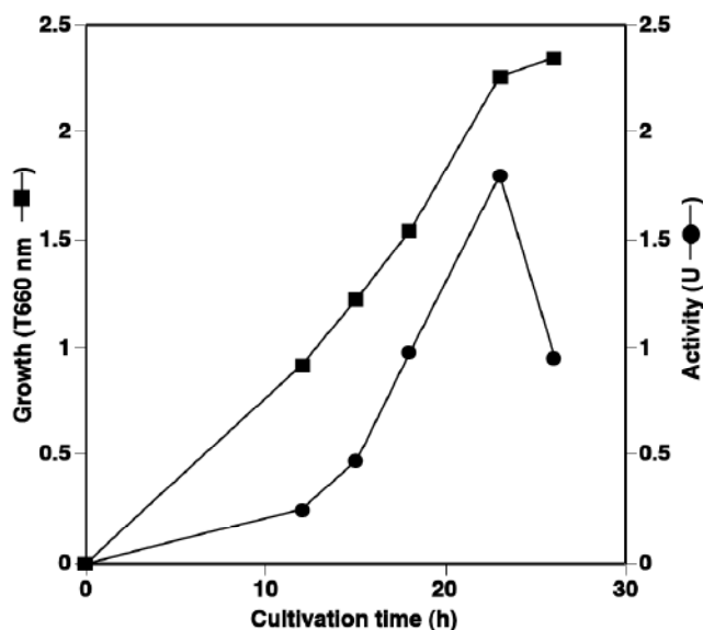
Fig. 2: Time course of the growth and homocholine dehydrogenase activity formation of Pseudomonas sp. strain A9. Cell-free extract was prepared from cells that grown on 300 ml of culture broth.
