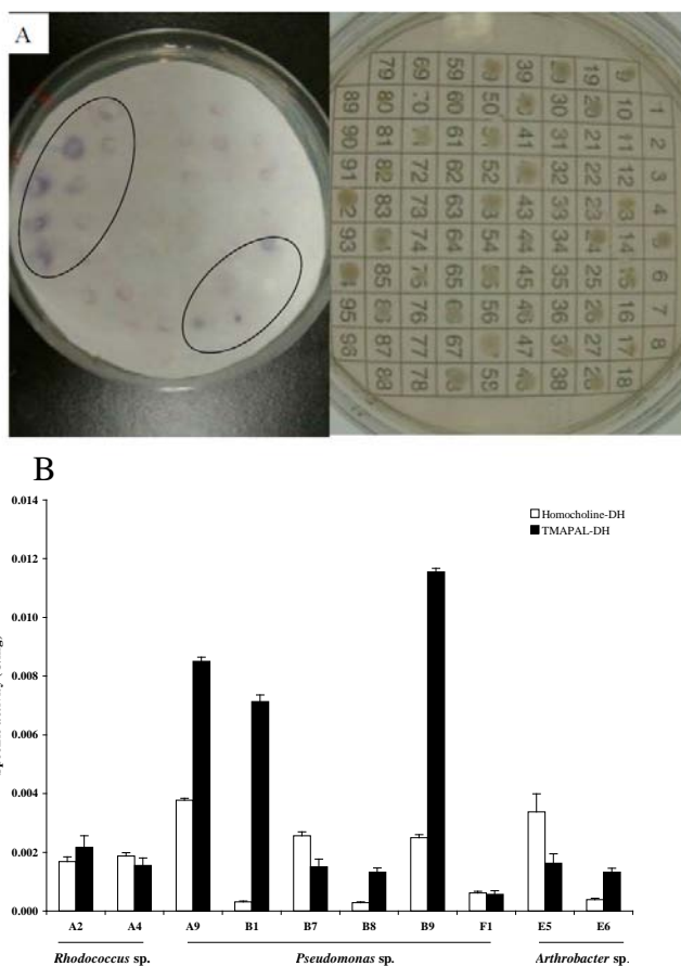
Fig. 1: Screening for dehydrogenases activity in the isolated strains by (A) replica staining and (B) spectrophotometric assays.
