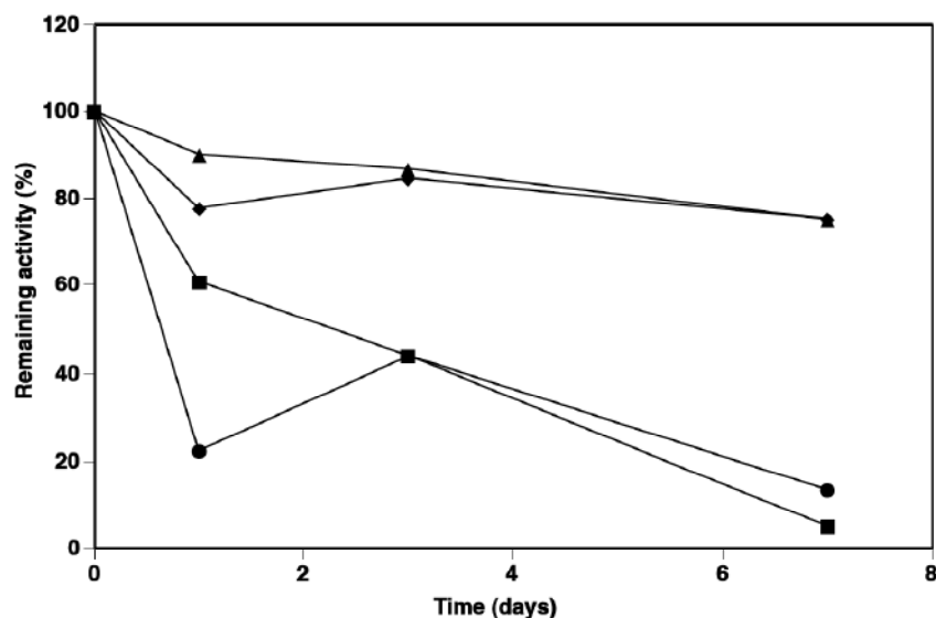
Fig. 3: Effect of stabilizers on the stability of homocholine dehydrogenase of Pseudomonas sp. strain A9. Cell free extract (1 ml) was dialyzed overnight against 50 mM potassium phosphate buffer containing either 1mM DTT (■), 1mM glutathione (●), 5% ethanol (▲), or 10% ethylene glycol (◆) and stored at 4°C for 1 week
