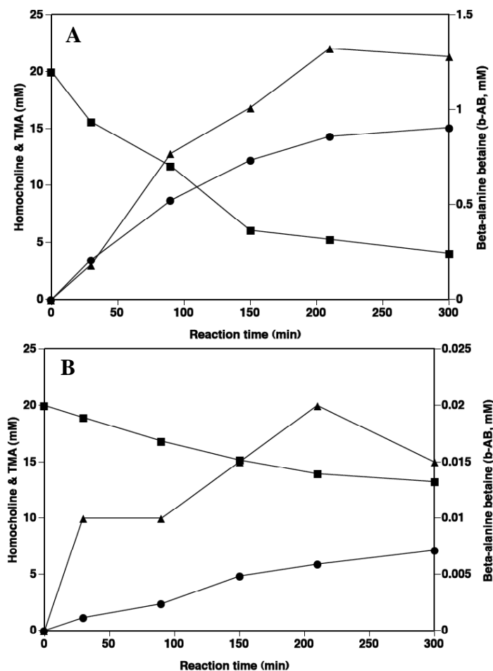
Fig. 6: Degradation of homocholine by dried cells of Pseudomonas sp. strain A9. Time course degradation of homocholine (■) and the generation of the metabolites beta-alanine betaine (▲) and TMA (●) by dried cells of Pseudomonas sp. strains A9. Dry cell reaction was performed with (A) and without (B) NAD + .
