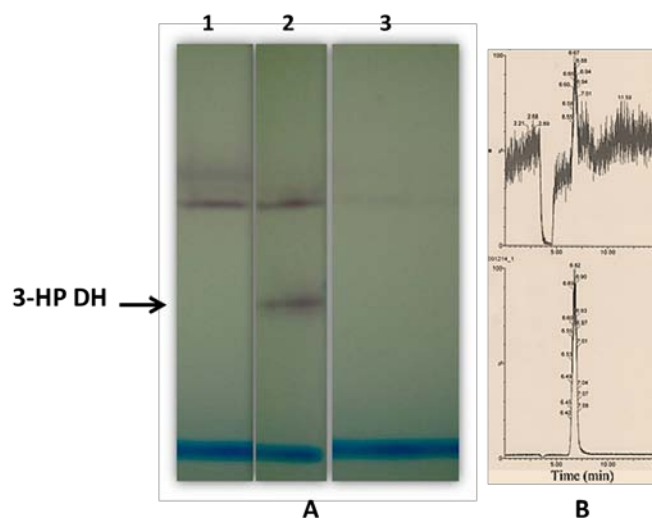
Fig. 7: (A) Non-denaturing gel (7.5% gel) stained for NAD + -dependent 3-hydroxypropionate dehydrogenase activity. Lane 1; homocholine-growing cells, lane 2; choline-growing cells, and lane 3; glucose-growing cells. (B) LC/MS/MS analysis of 3-hydroxypropionate in the degradation pathway of homocholine by the intact cells of Pseudomonas sp. Strain A9. Intact cell reaction mixture of strain A9 (upper) and authentic standard of 3-hydroxypropionate (lower).
