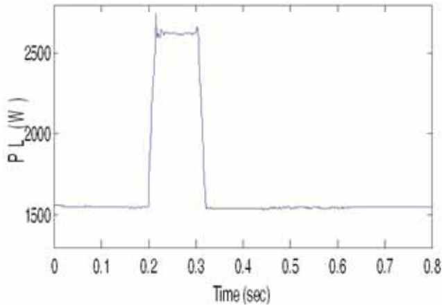
Fig. 9: Active power flowing through the circuit with fuzzy controller with RC load.
