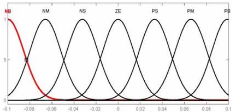
Fig.6. Membership Function of output (modulation index)
