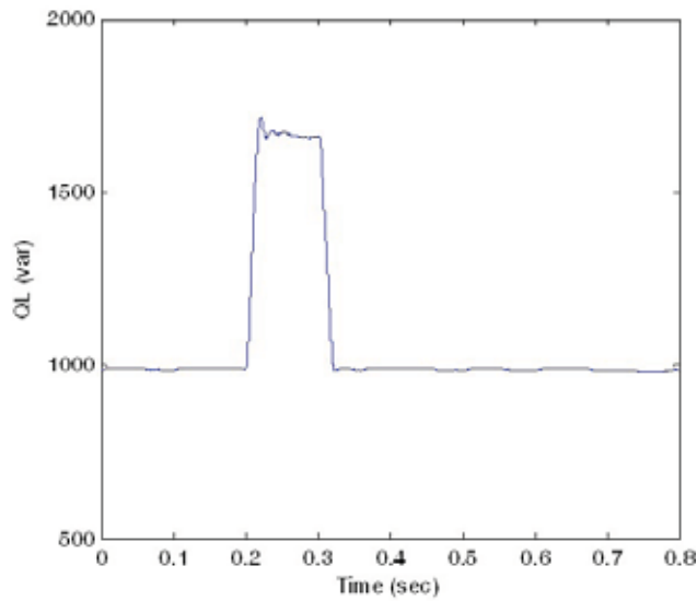
Fig. 20: Reactive power flowing through the circuit with conventional PI controller with RL load
