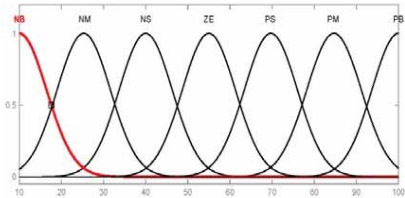
Fig. 4: Membership Function of error e(t)
