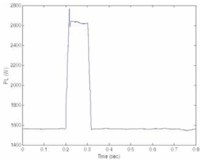
Fig. 13: Active power flowing through the circuit with conventional PI controller with RC load.
