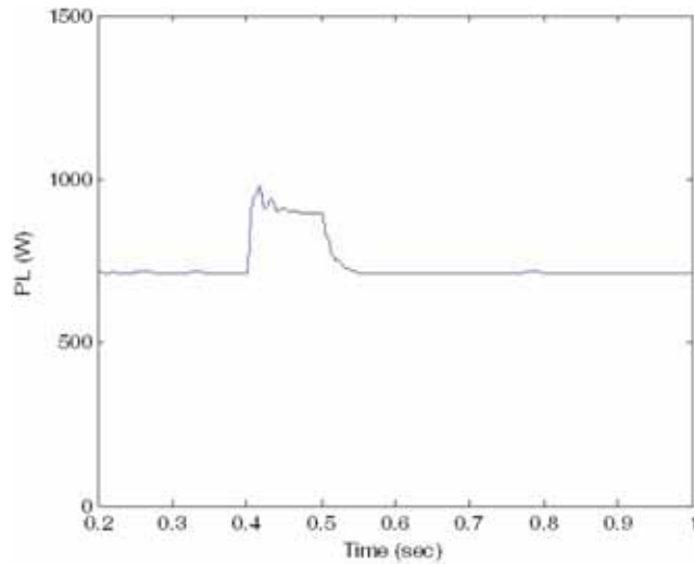
Fig. 17: Active power flowing through the circuit with fuzzy controller with RL load
