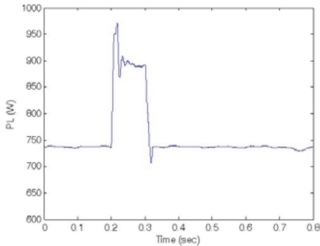
Fig. 21: Active power flowing through the circuit with conventional PI controller with RL load
