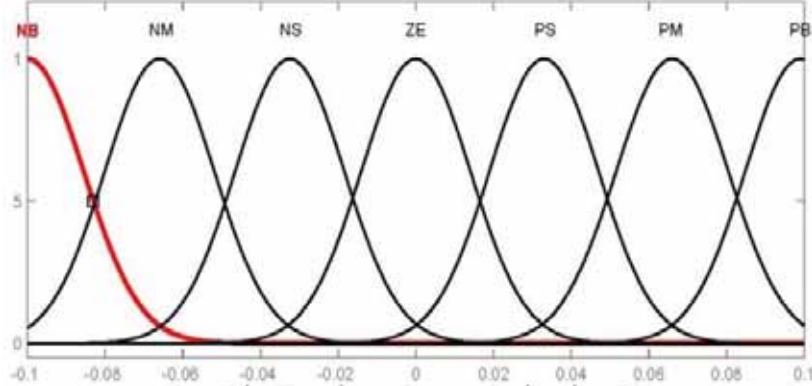
Fig. 5: Membership Function of error derivative \dot{e}(t)
