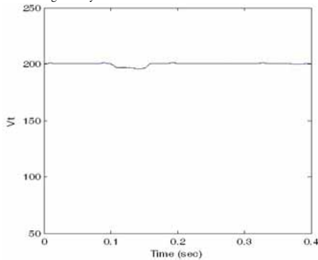
Fig. 19: The PCC voltage through conventional PI controller with RL load
