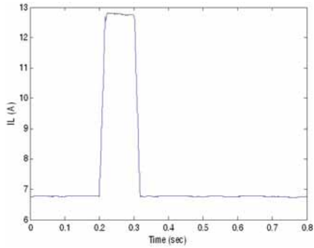
Fig. 14: The Load current through conventional PI controller with RC load.
