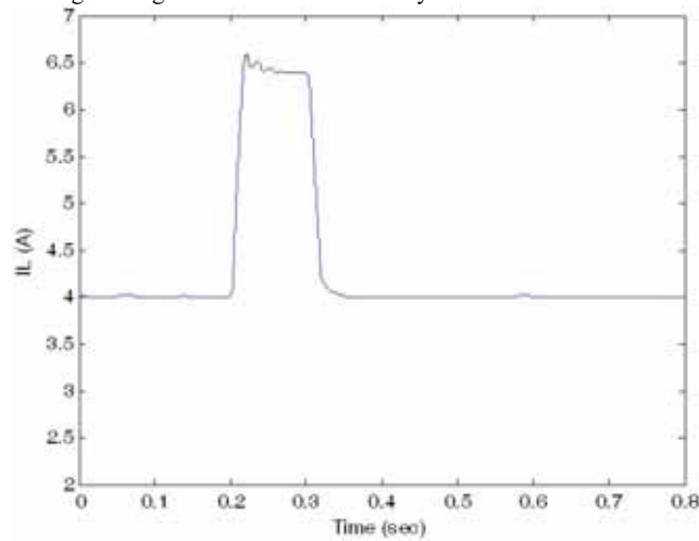
Fig. 18: The Load current through fuzzy controller with RL load
