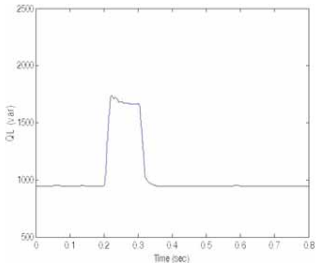
Fig. 16: Reactive power flowing through the circuit with fuzzy controller with RL load
