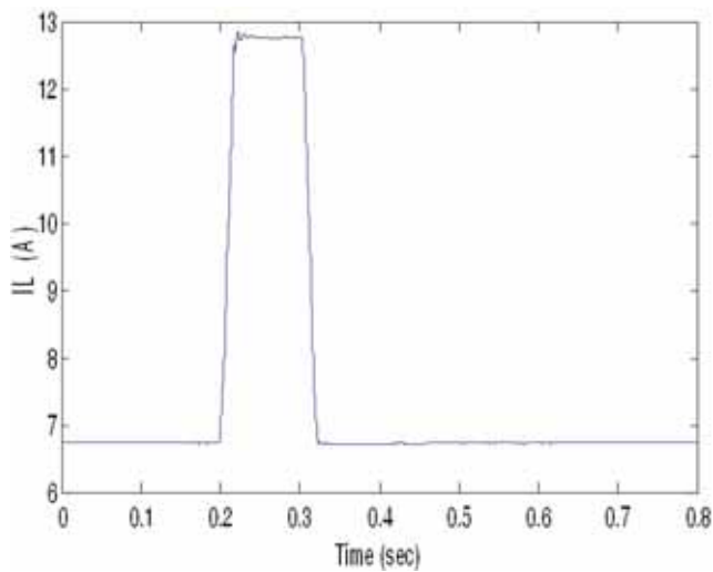
Fig. 10: The Load current through fuzzy controller with RC load.
