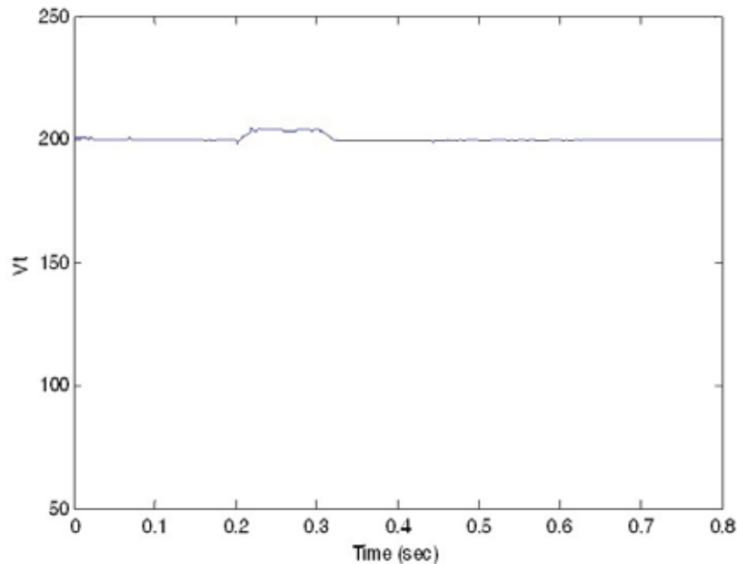
Fig. 7: The PCC voltage through fuzzy controller with RC load
