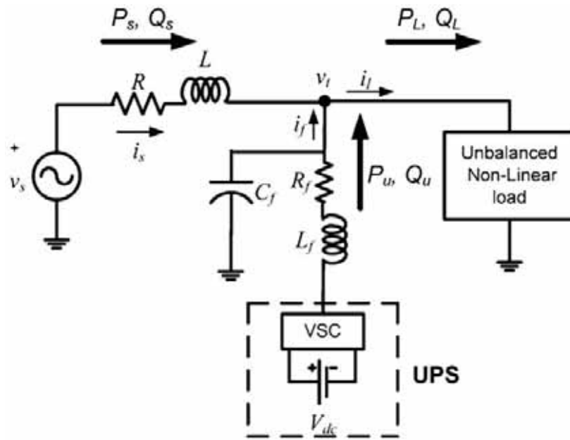
Fig. 2: Single-line diagram of the distribution system containing a UPS.
