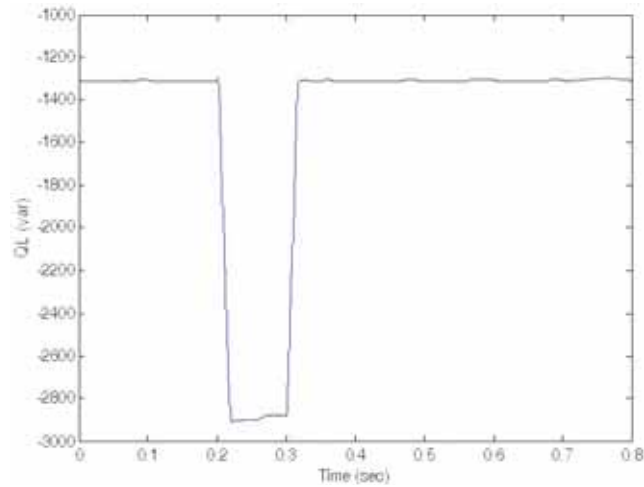
Fig. 12: Reactive power flowing through the circuit with conventional PI controller with RC load.
