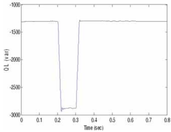
Fig. 8: Reactive power flowing through the circuit with fuzzy controller with RC load.
