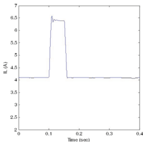
Fig. 22: The Load current through conventional PI controller with RL load.
