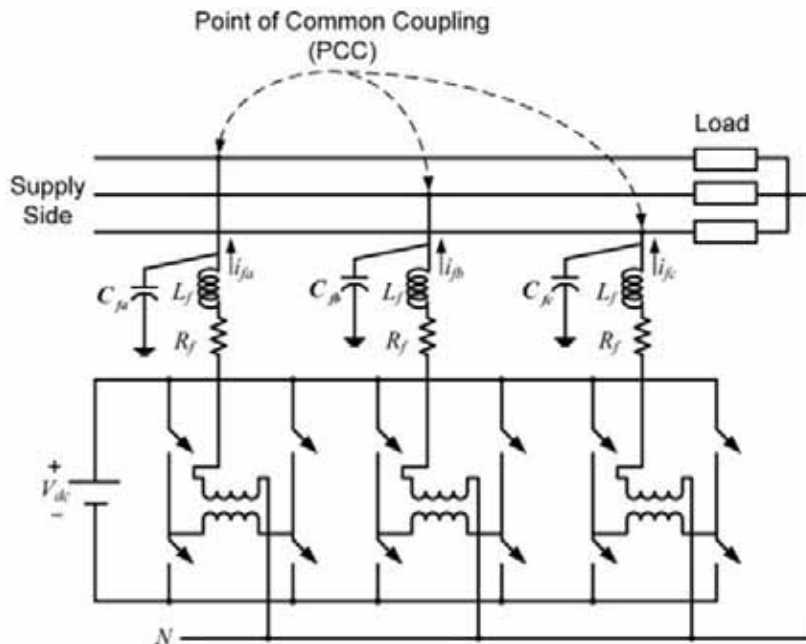
Fig. 3: UPS structure containing three VSCs that are supplied from a common dc source.
