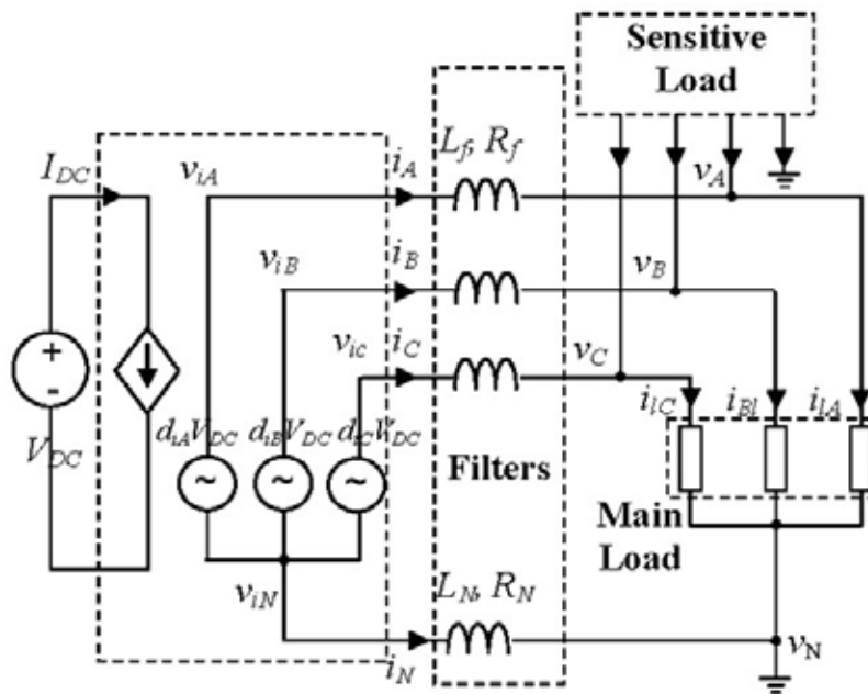
Fig. 1: Model of the three-leg VSI and the associated filters.
