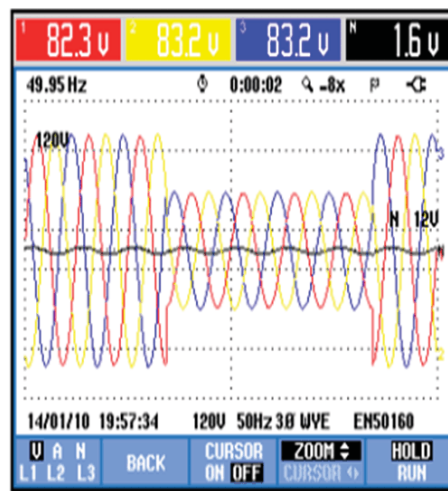
Fig. 5(a): Three phase fault Supply Voltages.
