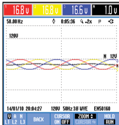
Fig. 5(a): Three phase fault Supply Voltages.
