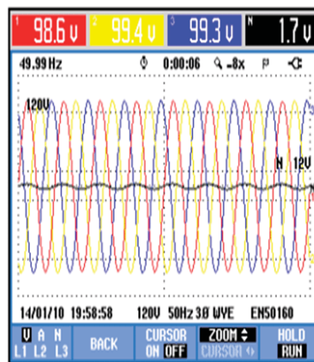
Fig. 6(a): Single phase fault Supply Voltages.
