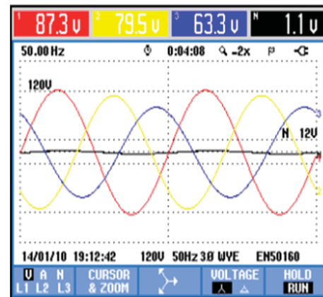
Fig. 7(a): Two phases fault Supply Voltages.
