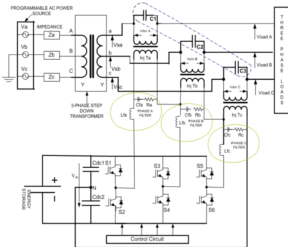
Fig. 4: The proposed new configuration of a DVR.
