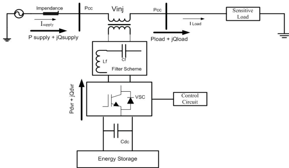
Fig. 1: Typical DVR circuit topology (single-phase representation).
