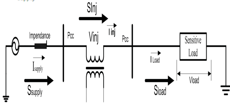
Fig. 2: Circuit diagram model of power system, controller and load.
