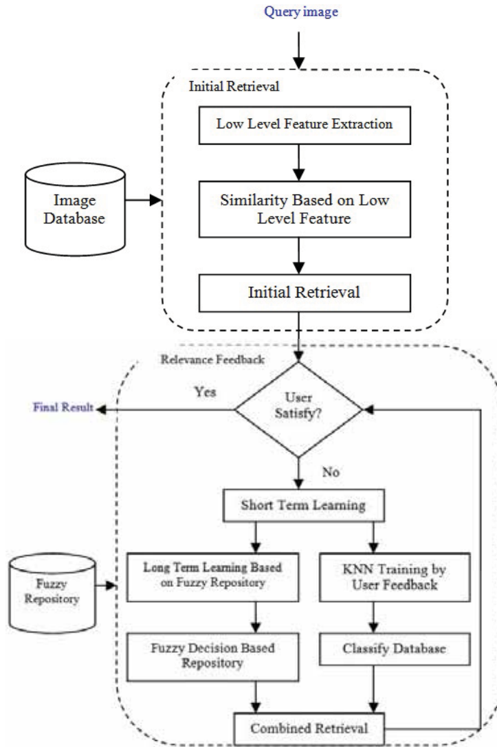
Fig. 2: The block diagram of our proposed system
