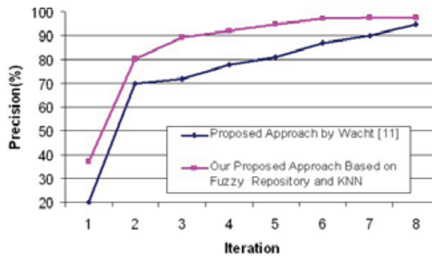
Fig. 8: Comparison of average precision between the proposed system and other system
