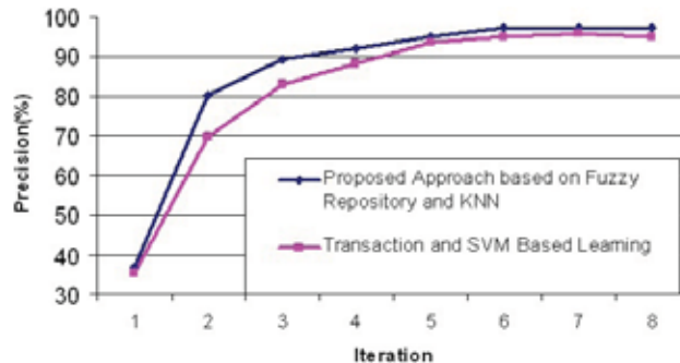
Fig. 9: Comparison of the proposed approach (fuzzy repository and KNN) and other approach (transaction and SVM based)
