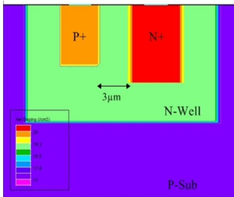
Fig. 6: PN Photodiode with width, W=3\ \mu\text{m} .
