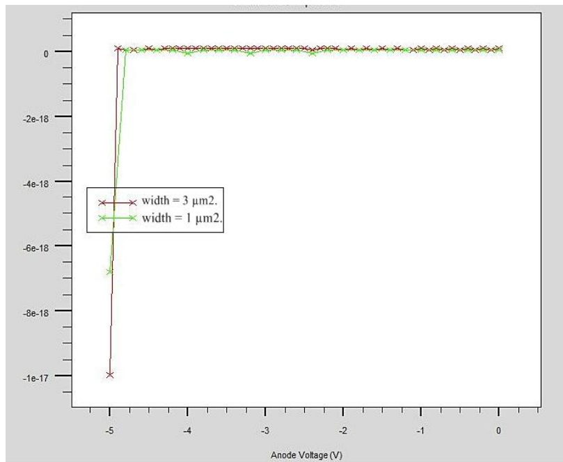
Fig. 8: I-V curve of PN Photodiode with different width.
