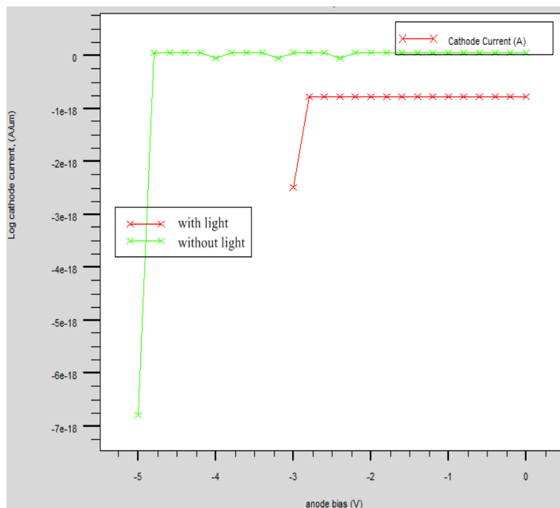
Fig. 10: I-V Curve of PN Photodiode with presence of light.
