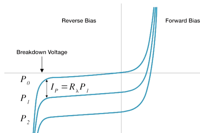
Fig. 3: IV Characteristics with different light level.
