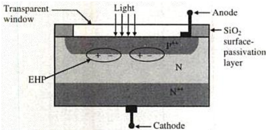
Fig. 1: PN Junction Photodiode.
