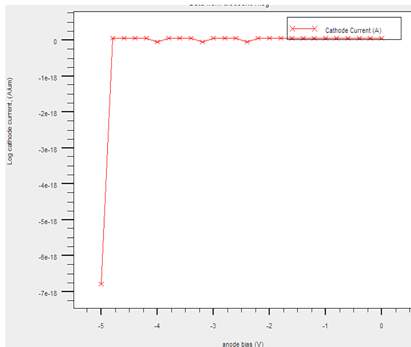
Fig. 9: IV curve for PN Photodiode without light.
