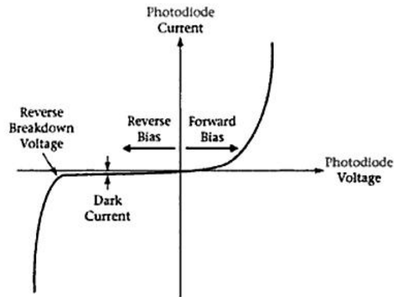
Fig. 2: IV Characteristic of PN photodiode.
