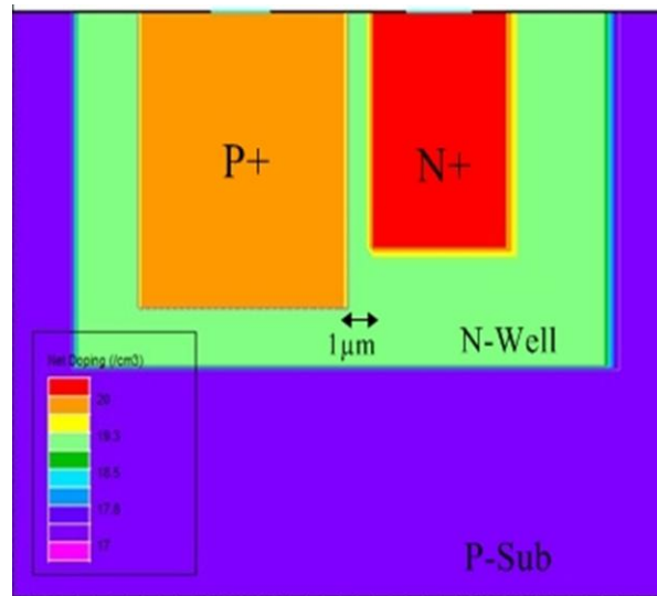
Fig. 4: PN Photodiode with width, W = 1 \mu\text{m} .
