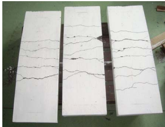
Fig. 4: Typical Crack Pattern on Reinforced Concrete Panels.
