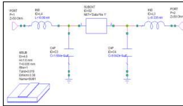
Fig. 7: Lumped Element Matching Network.
