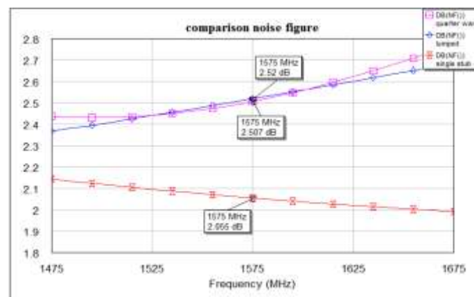
Fig. 10: Comparison of Noise Figure.
