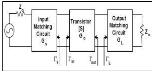
Fig. 3: The General Transistor Amplifier Circuit.
