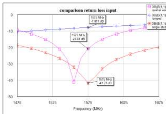
Fig. 8: Comparison Return Loss Input (S11).
