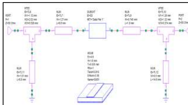
Fig. 5: Single Stub Matching Network.
