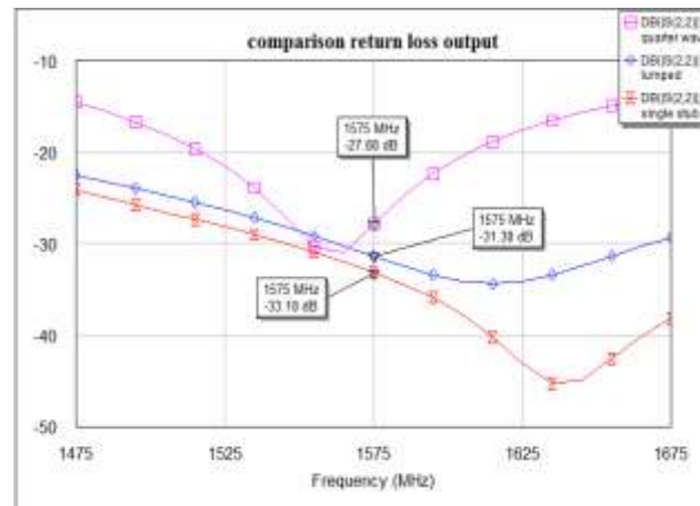
Fig. 9: Comparison Return Loss Output (S22).
